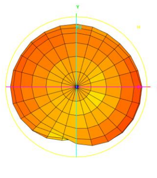
Total_3D_Side View 1_690MHz
