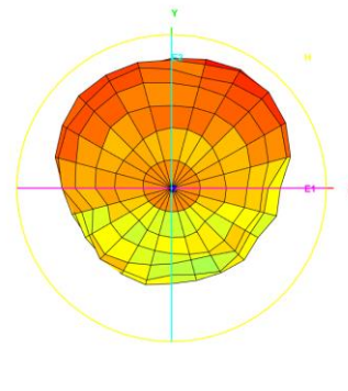
Total_3D_Side View 1_3.6GHz
