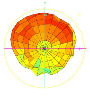
Total_3D_Side View 1_5.15GHz
