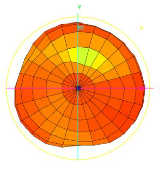
Total_3D_Side View_1_960MHz
