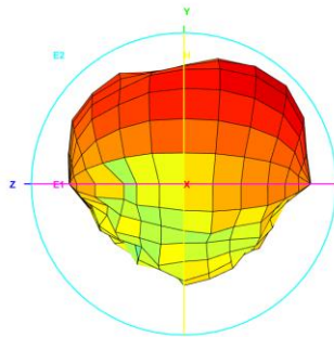
Total_3D_Top View_4.4GHz
