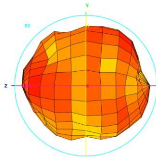
Total_3D_Top View_2.17GHz
