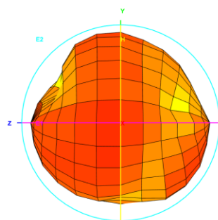
Total_3D_Top View_1.71GHz
