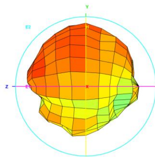
Total_3D_Top View_2.7GHz
