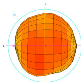
Total_3D_Top View_824MHz
