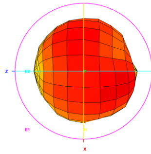
Total_3D_Left View_3.3GHz
