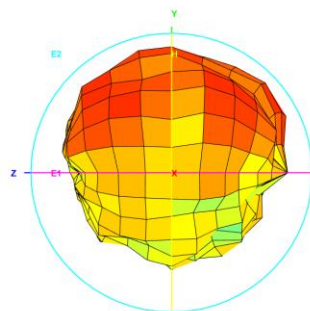
Total_3D_Left View_5.15GHz
