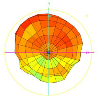
Total_3D_Side View 1_2.6GHz
