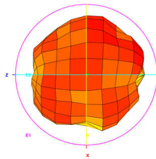
Total_3D_Left View_5.15GHz
