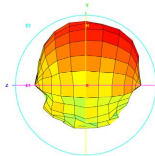
Total_3D_Top View_3.6GHz
